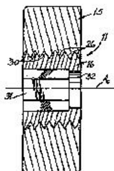
Figs. 3 & 6 of the '007 patent (back and cross-sectional views)
