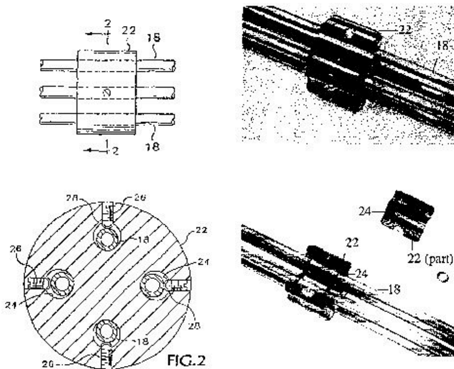
Adjustment Member of the '325 patent (Assembled and cross-sectional views)
